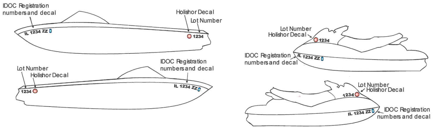
Figure 1: Decal Placement
